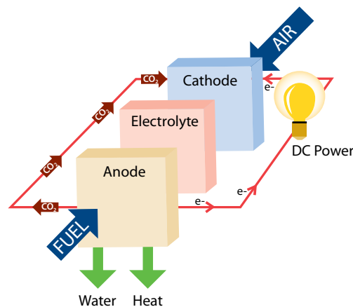
Figure 1: How a Molten Carbonate Fuel Cell Works
